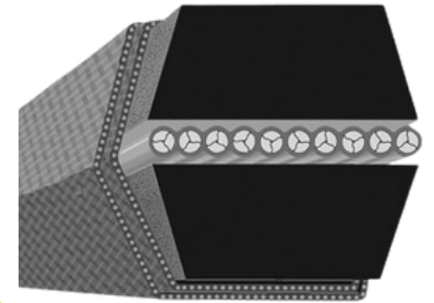
Double V-Belts
